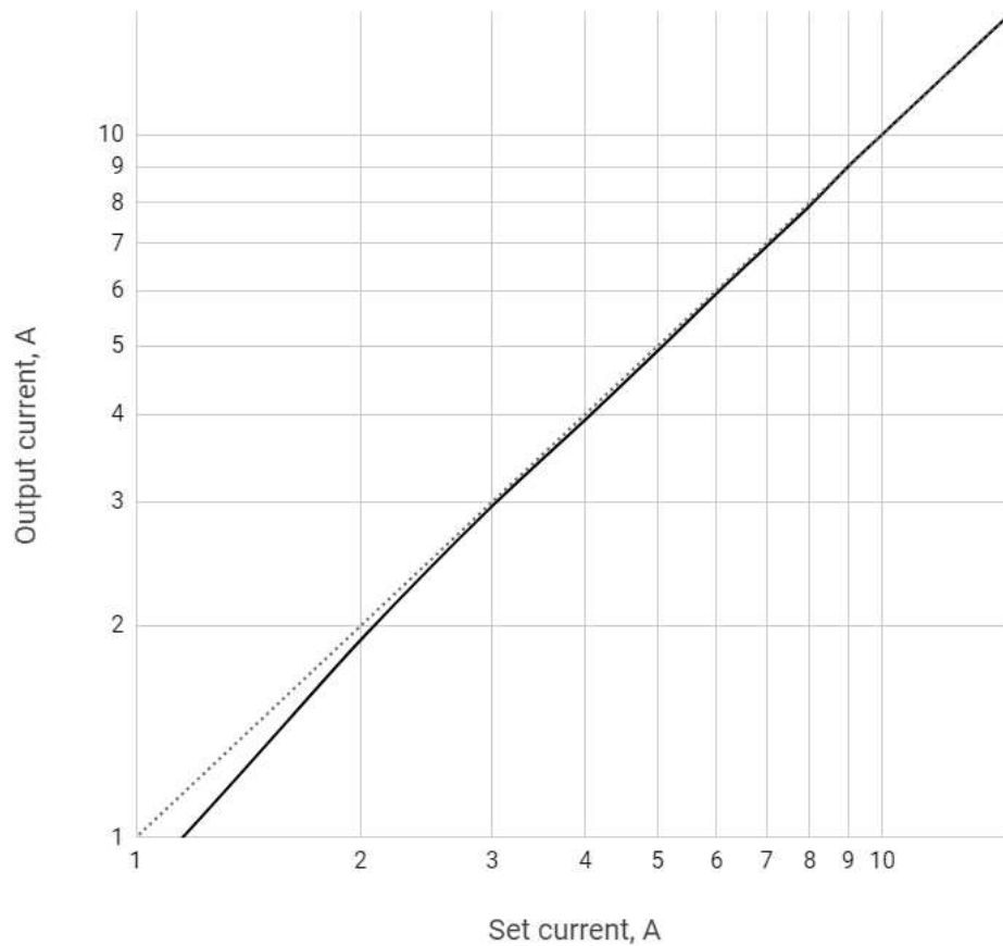
Figure 5 – Regulation characteristic: dotted – ideal, solid – real
