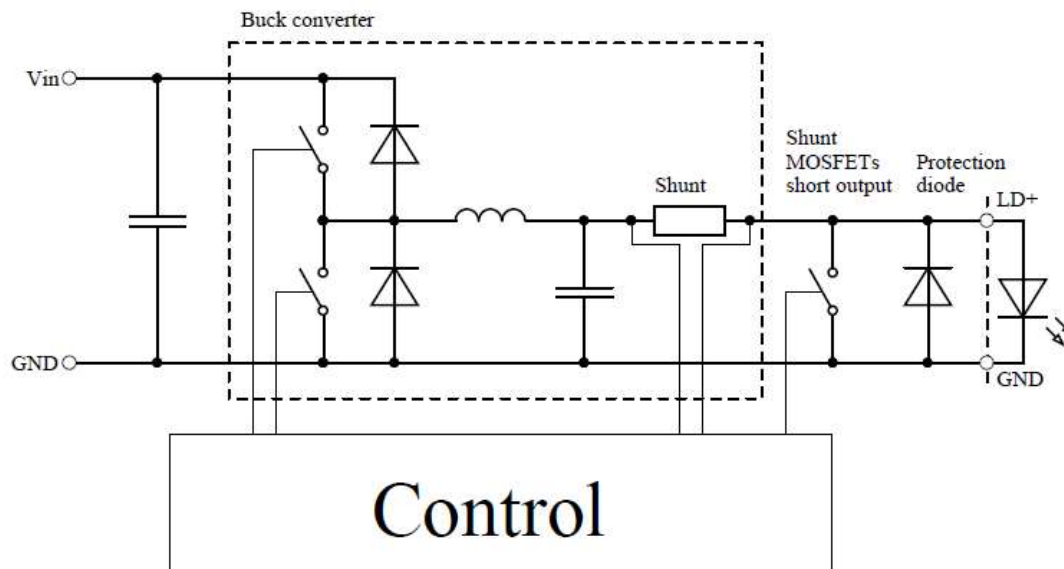
Figure 9 – Power unit functional scheme
