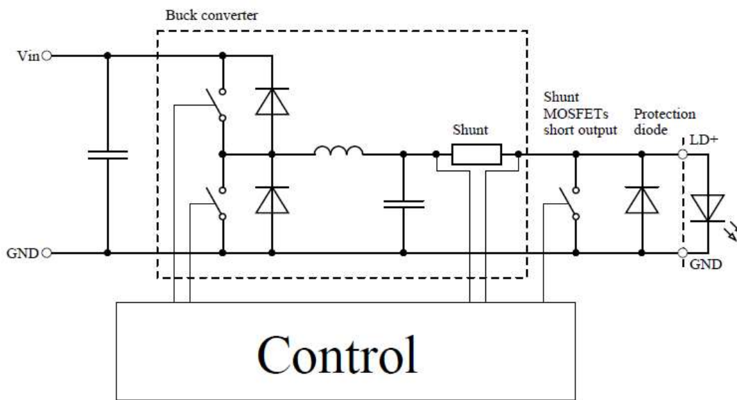
Figure 9 – Power unit functional scheme
