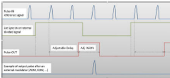
Pulse picking principle (mode : Divider or Synchro).
