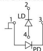
PINOUT #12
